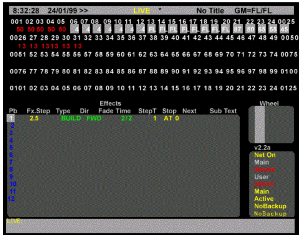
The Live Screen - Effects Window - GeniusPro
